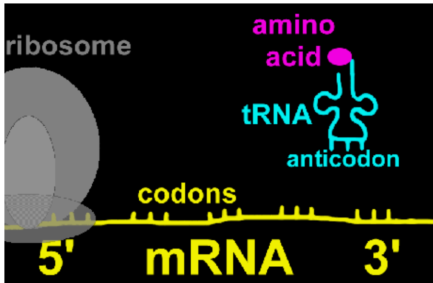
tRNA molecule
